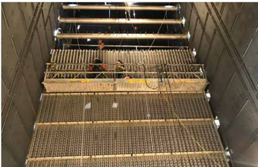
Distribution Grid Layout (looking downstream of gas flow)
