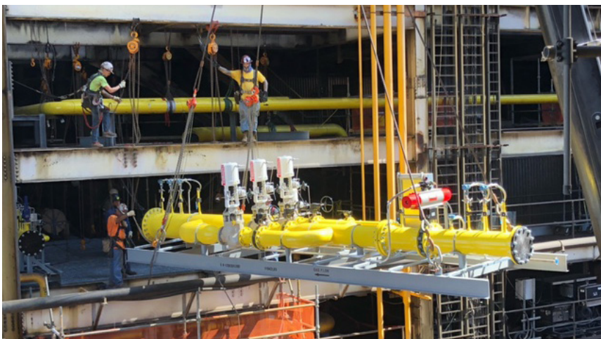
Pressure Control and Flow Control Skid
