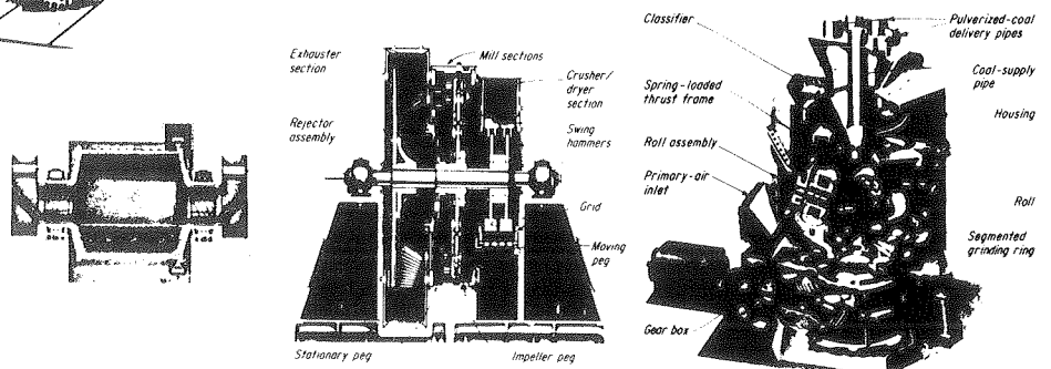
Three common types of coal pulverizers
