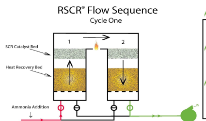
Figure 1: Operation of a two-canister RSCR design.
