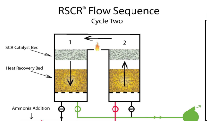
Figure 2: RSCR flow sequence – cycle two
