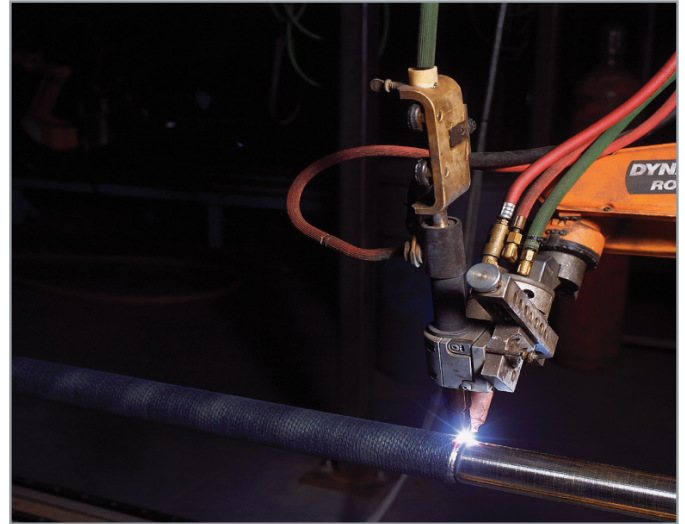
The Patented Wave Pulse Technology System utilizes state-of-the-art robots and assures consistent weld metal disposition.
